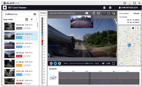
Windows/macOS Viewer
